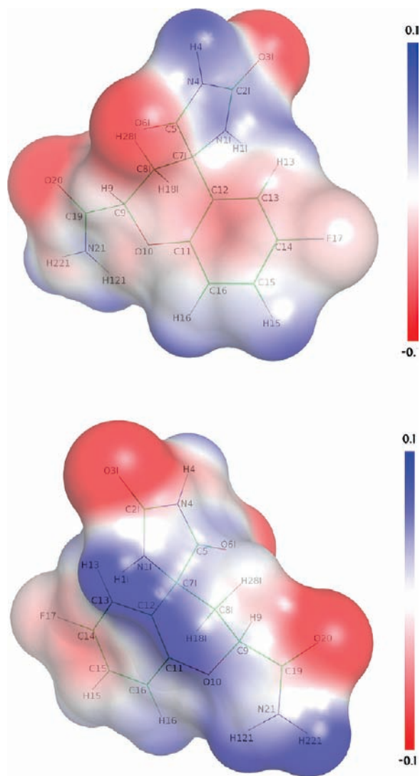
Figure 7. Deformation electrostatic potential \Delta\varphi ( e/\text{\AA} ) generated by the isolated fidarestat molecule mapped on the solvent-excluded surface with a probe radius of 1.4 \text{\AA} . The potential \Delta\varphi is derived from the deformation electron density \Delta\rho . The view was made with program Pymol. 69
