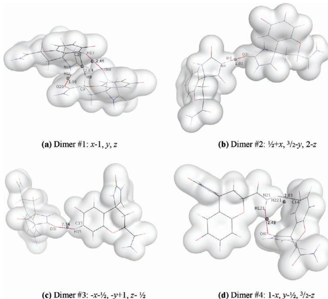
Figure 4. View of the four different hydrogen bonded dimers of fidarestat molecules found in the crystal packing with their corresponding symmetry operators. The gray surfaces represent the experimental electron density iso-contour with a cutoff value of +0.05 e/\text{\AA}^3 . Red, purple, and gray dashed lines represent H-bonds, weak contacts, and H... \pi -system bonds, respectively. Gray spheres represent intermolecular BCPs. The view was made with program Pymol. 69
