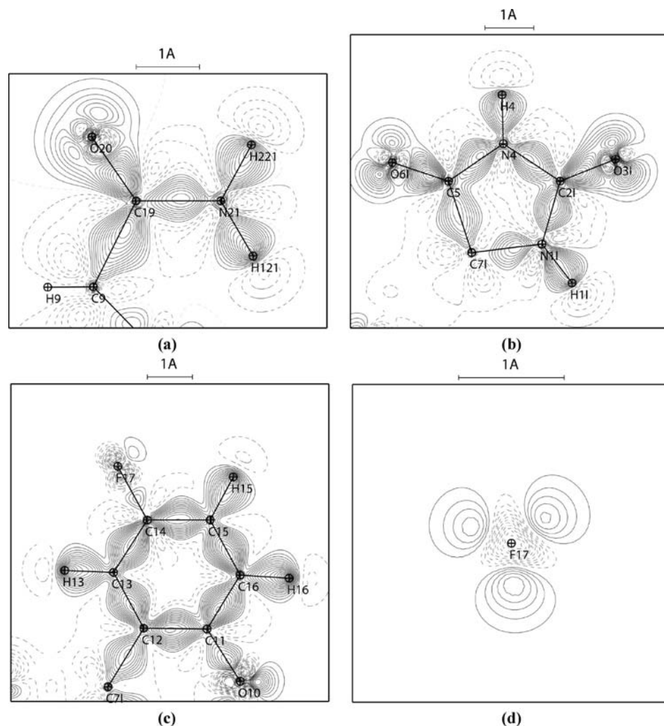
Figure 5. Experimental static deformation electron density maps in the planes of (a) the carbamoyl moiety, (b) the hydantoin ring, and (c) the fluorophenyl-like moiety of the chroman ring. In (d) the plane is perpendicular to the F17–C14 bond, outside of the F17–C14 segment at a distance of 0.1 Å to the fluorine atom. The vertical direction is perpendicular to the phenyl ring plane. Contours intervals are \pm 0.05 \text{ e}/\text{\AA}^3 , positive and negative in continuous and dashed lines, respectively.
