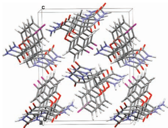
Figure 2. View along the a axis of the crystal packing of the fidarestat molecule. The view was drawn using Mercury software. 68
