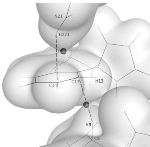
Figure 8. View of the hydrogen bonds with \pi acceptors in a trimer of fidarestat molecules. The aromatic ring containing the C13–C14 atoms is involved on both sides in H... \pi -system bonds represented as gray dashed lines. The electron density cutoff value for the iso-surface is +0.05 e/Å 3 . The view was made with program Pymol. 69
