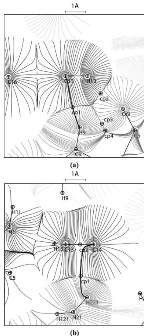
Figure 9. Gradient lines of the total electron density in the regions of the hydrogen bonds with \pi acceptors. In the planes defined by the atoms C13, H13 and H9 (a), and by the atoms C13, C14 and H221 (b). The most interesting CPs are indicated. The views were made using the VMOPro software. 22 Intermolecular bond paths are added with bold black lines.
