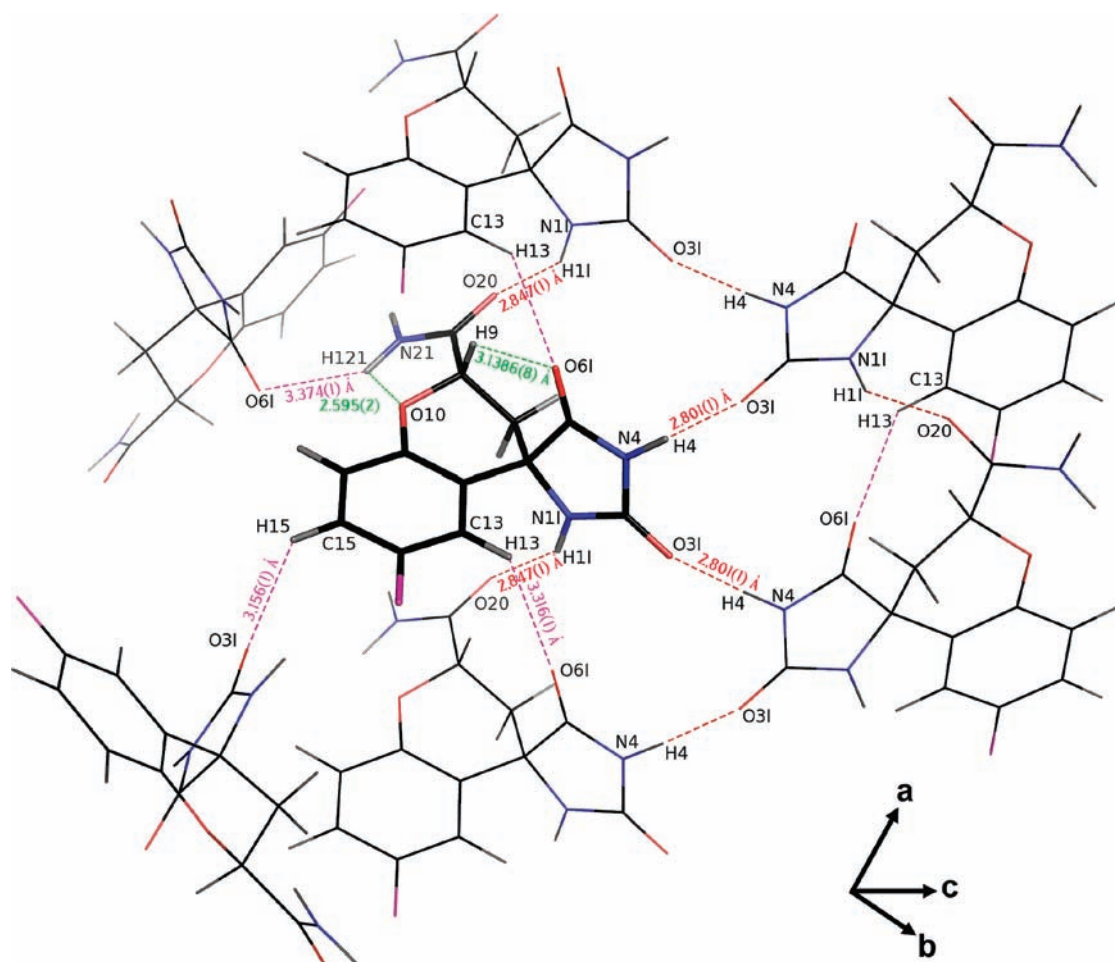
Figure 3. Crystal packing diagram for fidarestat, showing the network of hydrogen bonds (dashed lines). The view was made with program Pymol. 69
