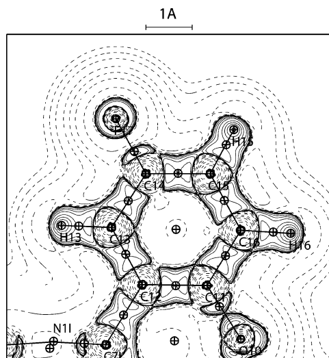
Figure 6. Experimental Laplacian \nabla^2\rho distribution maps in the planes of the fluorophenyl-like moiety of the chroman ring. Solid lines show negative contours, and dashed lines show positive contours. Contours intervals are semilog \pm 0.2, 0.4, 0.8, 2.0 \dots e/\text{\AA}^5 . The positions of the bond and ring critical points are also shown.
