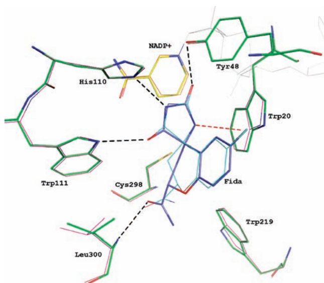
Figure 10. Main interactions between hAR active site residues and fidarestat stereoisomers. The conformations of hAR complexed with fidarestat (in thick lines) and its hAR-(2 R ,4 S ) isomer (in fine lines) are superimposed. The hydrogen bonds are represented in black dash lines, except the H... \pi hydrogen bond which is in red dash line. The view was made with program Pymol. 69
