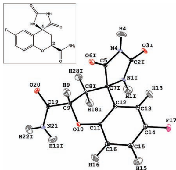
Figure 1. OrtepIII representation 67 of fidarestat with thermal displacement ellipsoids plotted at 50% probability and chemical diagram of fidarestat in frame.
